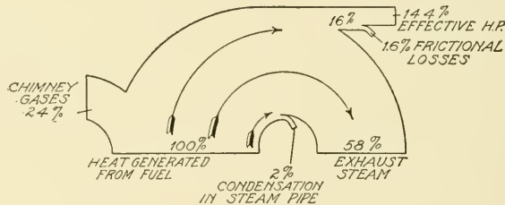
Fig. 143. Diagram Showing Heat and Other Losses in Power Plant
